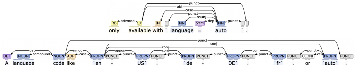
Figure 4: Parsed dependency graphs of preferredVariants parameter description (top) and language parameter description (bottom) from Languagetool’s OpenAPI specification.
