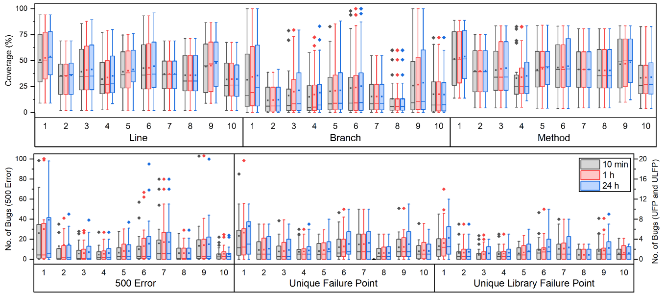
Figure 2: Code coverage achieved and number of unique 500 errors, unique failure points, and unique library failure points detected over all services by the ten tools in 10 minutes, 1 hour, and 24 hours (1: EvoMasterWB, 2: RESTler, 3: RestTestGen, 4: RESTest, 5: bBOXRT, 6: Schemathesis, 7: Tcases, 8: Dredd, 9: EvoMasterBB, 10: APIFuzzer).
